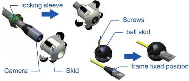
Figure 16. 134 Roller skid
