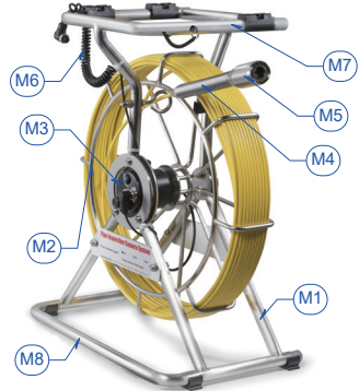
Figure 9. Frame assembly
