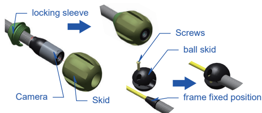
Figure 15. 78 Roller skid
