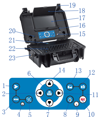
Figure 6.Toolbox unit
