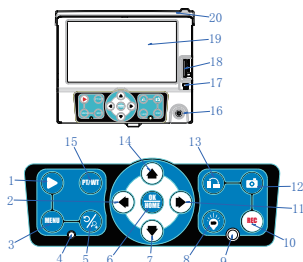
Figure 4.DVR
